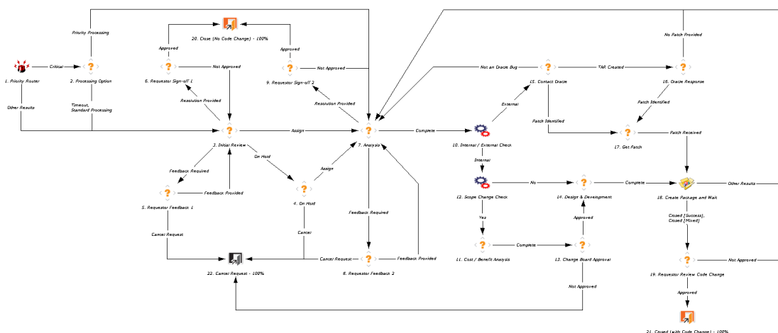
Figure 5-1. OraApps Application Issue workflow
