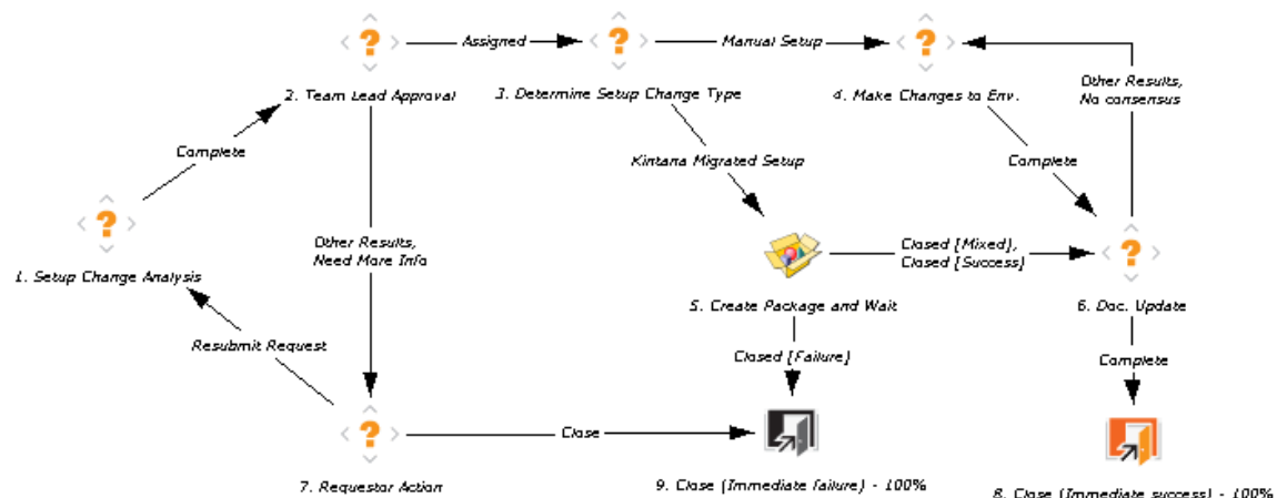
Figure C-13. OraApps Setup Change Process workflow
