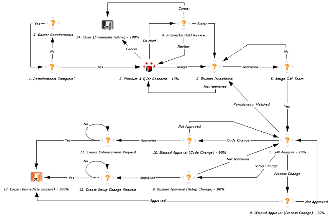
Figure C-7. OraApps GAP Analysis Process workflow
